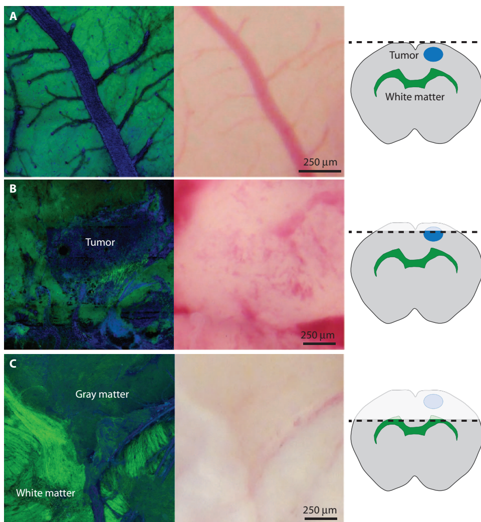
Fig. 6. SRS imaging during simulated tumor resection on mouse brain. En face , epi-SRS images were obtained in vivo during various stages of a simulated tumor removal. The cartoons on the right show the depth of imaging. (A) In a tumor located beneath the cortical surface, there is no obvious abnormality in SRS (left) or bright-field images (middle) when imaging the cortical surface. (B) After a portion of the cortex has been removed, the tumor is revealed. Blood was present on the dissected surface but did not adversely affect the distinction of tumor-infiltrated regions from non-infiltrated regions. (C) Because dissection was carried deep past the tumor, the normal appearance of white matter and cortex was again visible.
